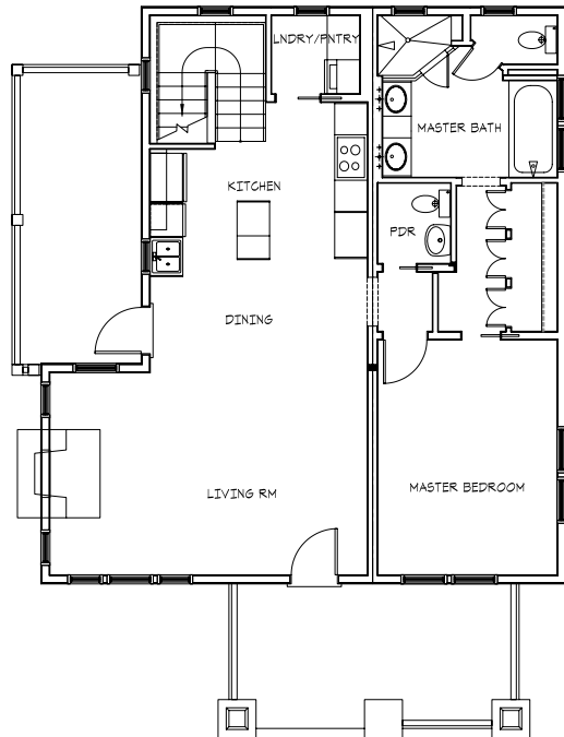
FIRST FLOOR PLAN 1,002 Square Feet
