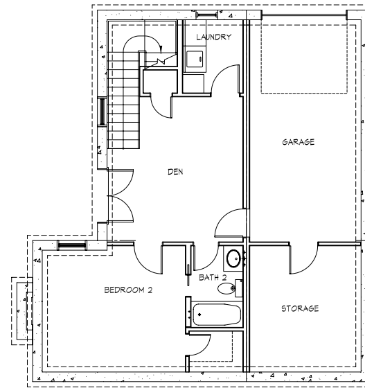
BASEMENT FLOOR PLAN 494 Finished Square Feet
